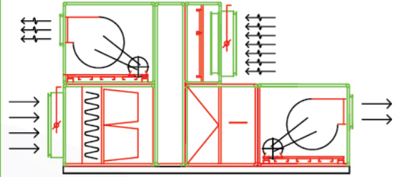
2 FRESH AIR HANDLING UNIT INSTALLATION
