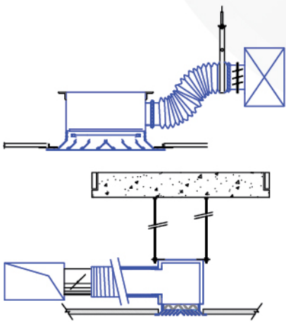
5 AIR OUTLETS INSTALLATION
