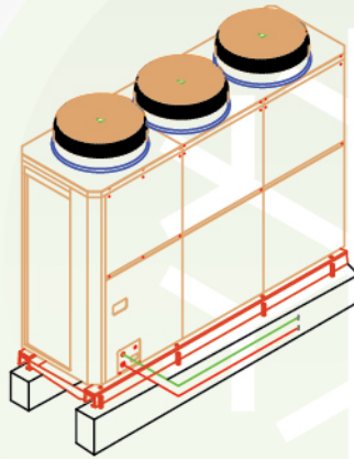
3 DX DECORATIVE TYPE & VRF UNITS INSTALLATION
