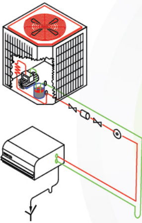
3 DX DECORATIVE TYPE & VRF UNITS INSTALLATION
