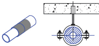
6 CHILLED WATER PIPE INSTALLATION
